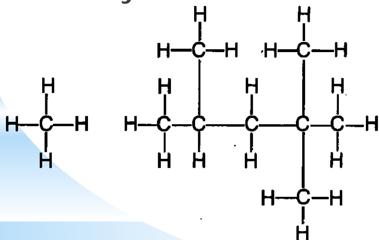
Methane
