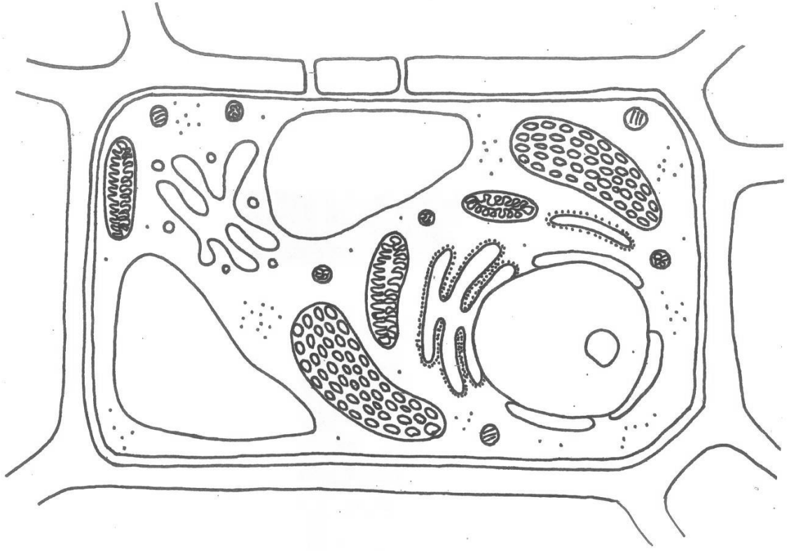
Plant Cell
